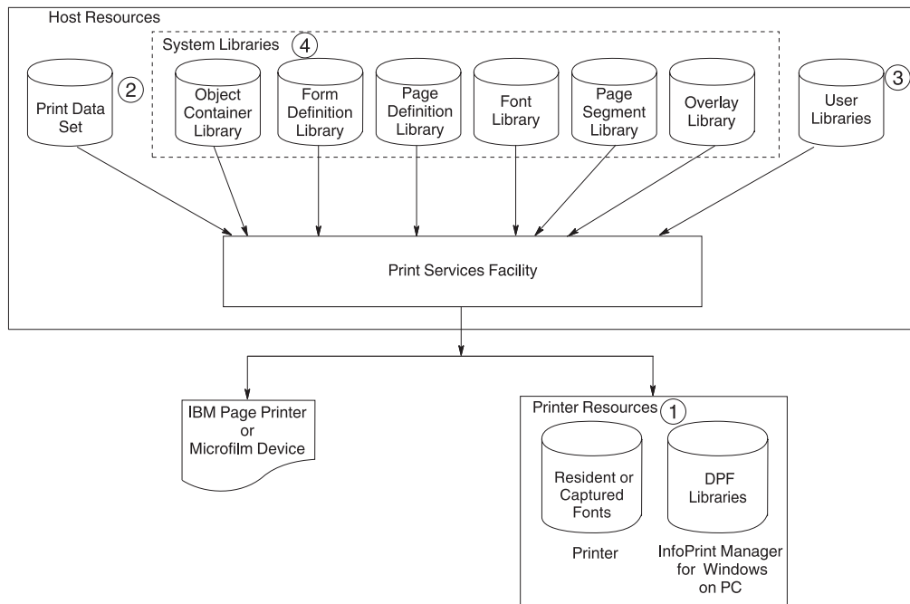
Figure 8. Resource Storage
